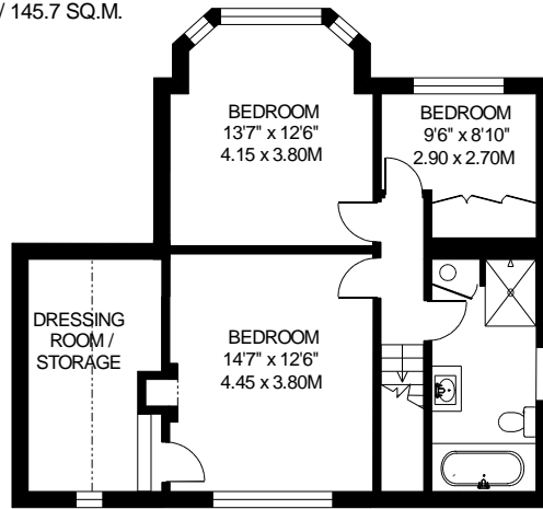
FIRST FLOOR 710 SQ.FT.
